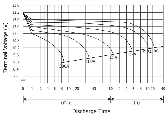
Discharge Curves 77°F(25°C)
